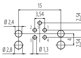
Winkelversion/Angled version
