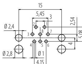
Winkelversion/Angled version
