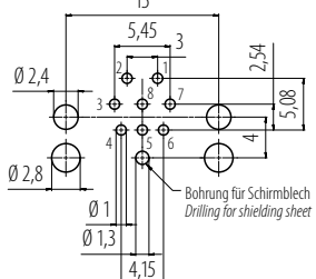
Winkelversion/Angled version
