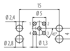
Winkelversion/Angled version
