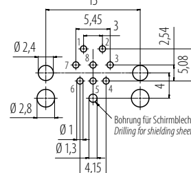
Winkelversion/Angled version
