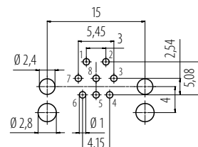
Winkelversion/Angled version
